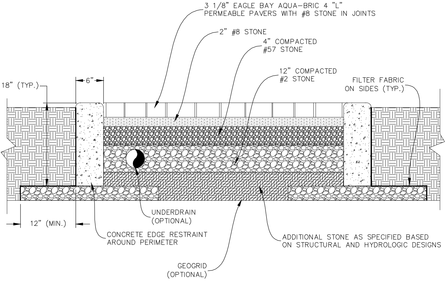
TYPICAL SECTION 'A-A' NTS
